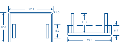
Tapa final
