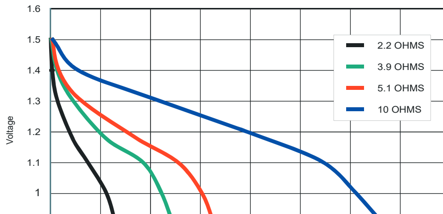
TYPICAL DISCHARGE CHARACTERISTICS AT 21 °C (70 °F)
