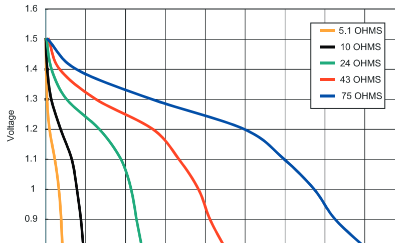
TYPICAL DISCHARGE CHARACTERISTICS AT 21°C (70°F)
